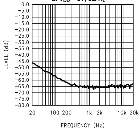
Figure 10. Input terminated with 10\Omega
