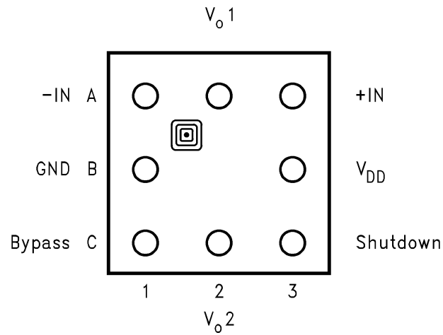
8 Bump DSBGA (Top View) See Package Number YZR
