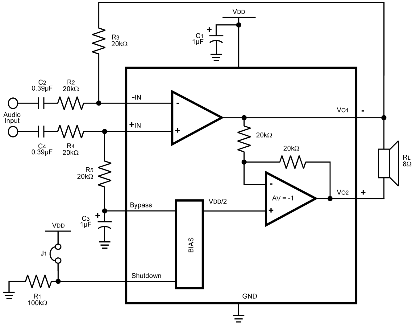
Figure 32. DIFFERENTIAL AMPLIFIER CONFIGURATION FOR LM4904
