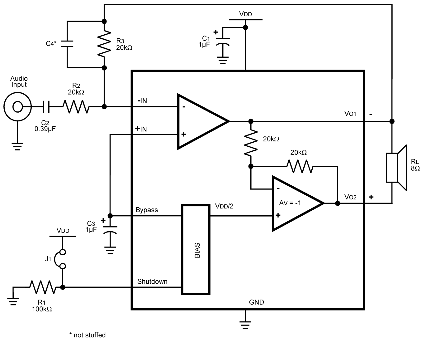
Figure 33. REFERENCE DESIGN BOARD SCHEMATIC
