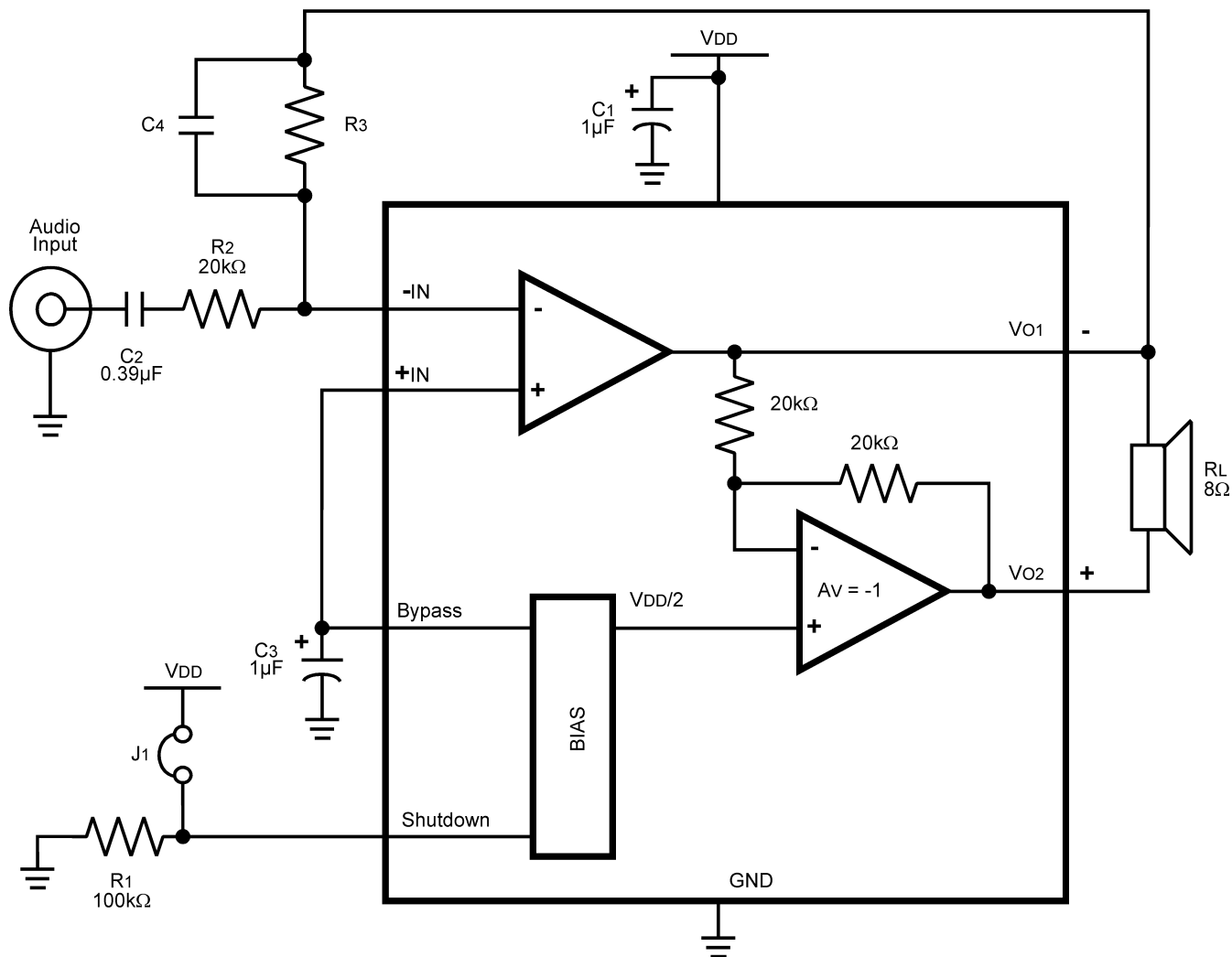
Figure 31. HIGHER GAIN AUDIO AMPLIFIER
